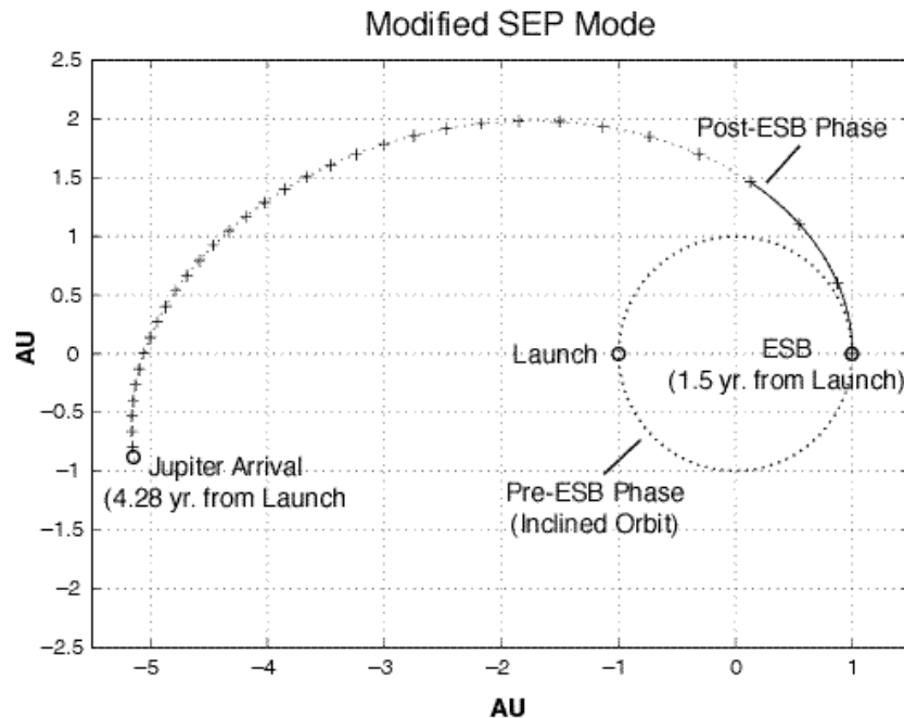
Figure 7. Jupiter Mission Trajectory with Out-of-Ecliptic Initial Thrust Phase Tick Marks indicate 30-Day Intervals (Example V_{rel} = 6 km/sec at End of Pre-ESB Phase).
