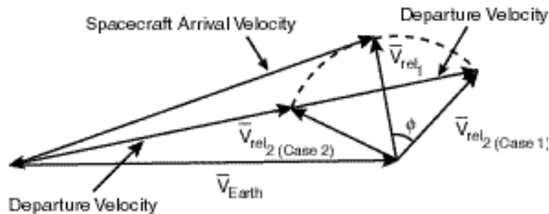
* Results of Earth Swingby Maneuver in 2 Dimensions
