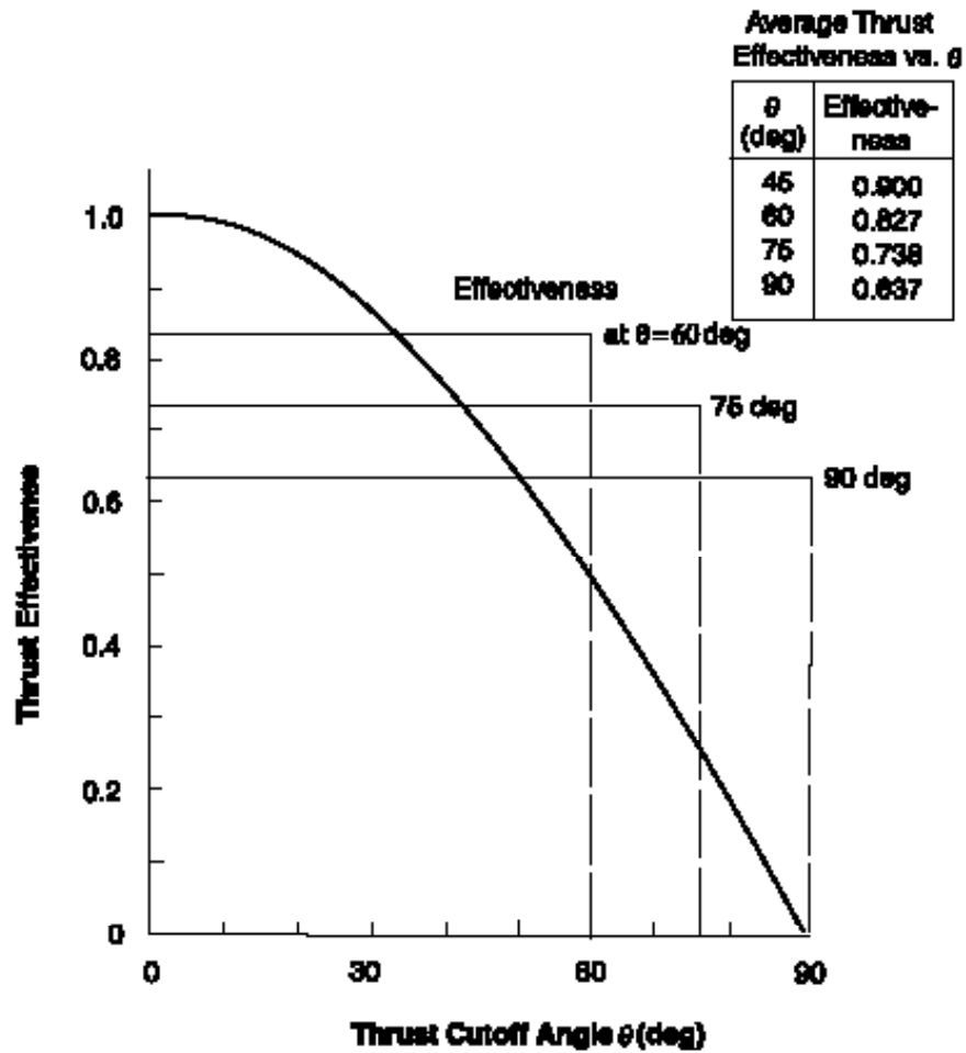
Figure 2. Average Thrust Effectiveness for Several Cutoff Angles.
