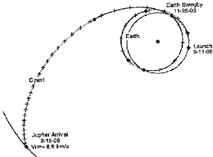
Figure 3. SEP Earth Gravity Assist Jupiter Orbiter Trajectory With In-Ecliptic Pre-ESB Thrust Phase (from Ref. 2) Tick Marks Indicate 30 Day Intervals.
