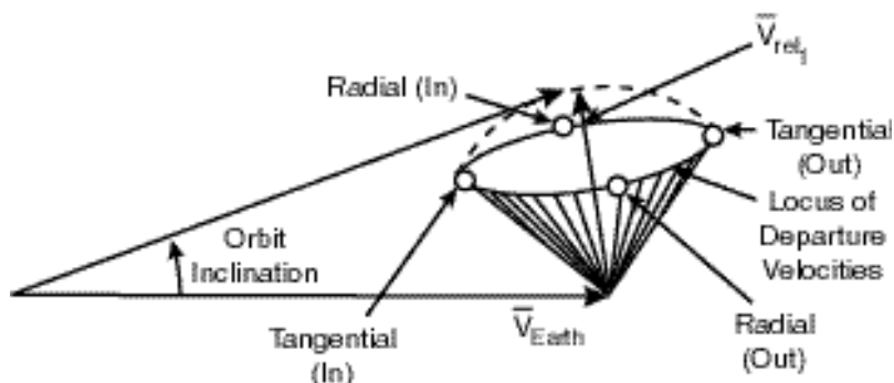
* Results of Earth Swingby Maneuver in 3 Dimensions
