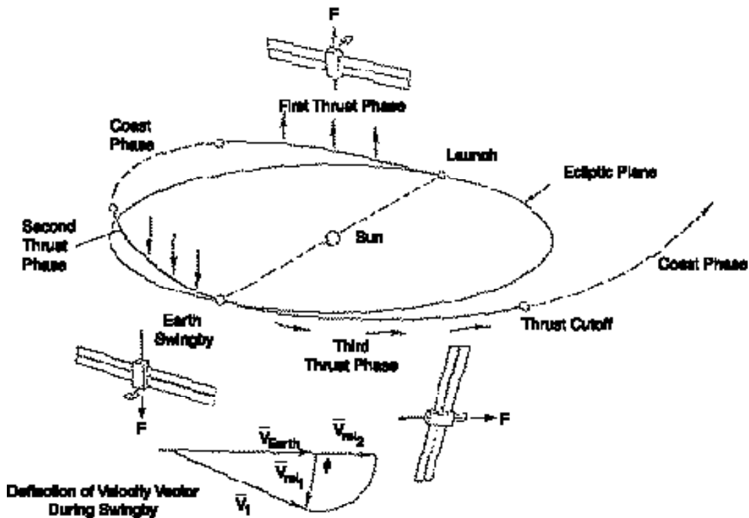
Figure 1. Outer Planet Mission with Earth Swingby: Mission Profile and Thrust Pointing Requirements.
